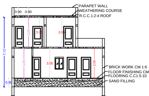
SECTION ON SV
