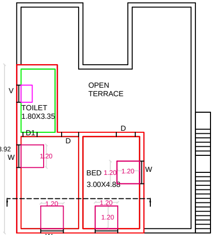
PRPOSED FIRST FLOOR
