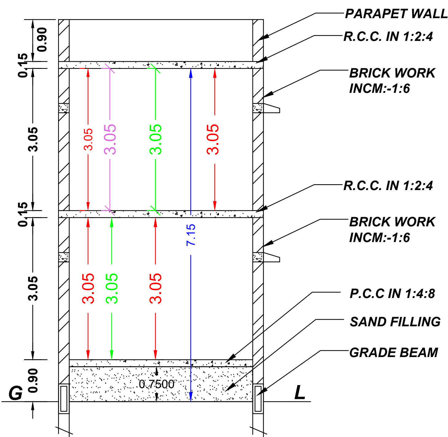
SECTION "AB"
