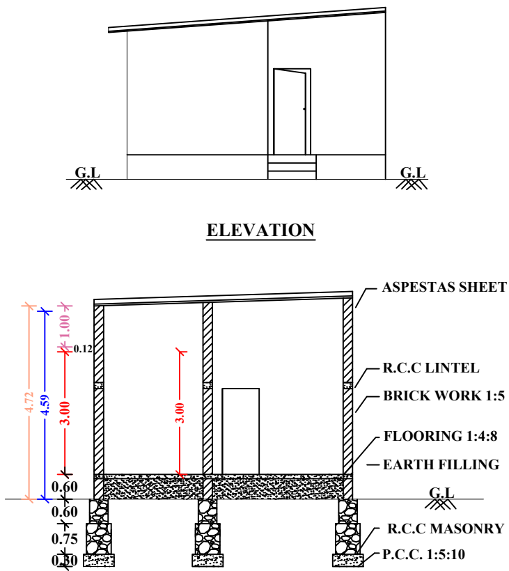
"SECTION "AB"
