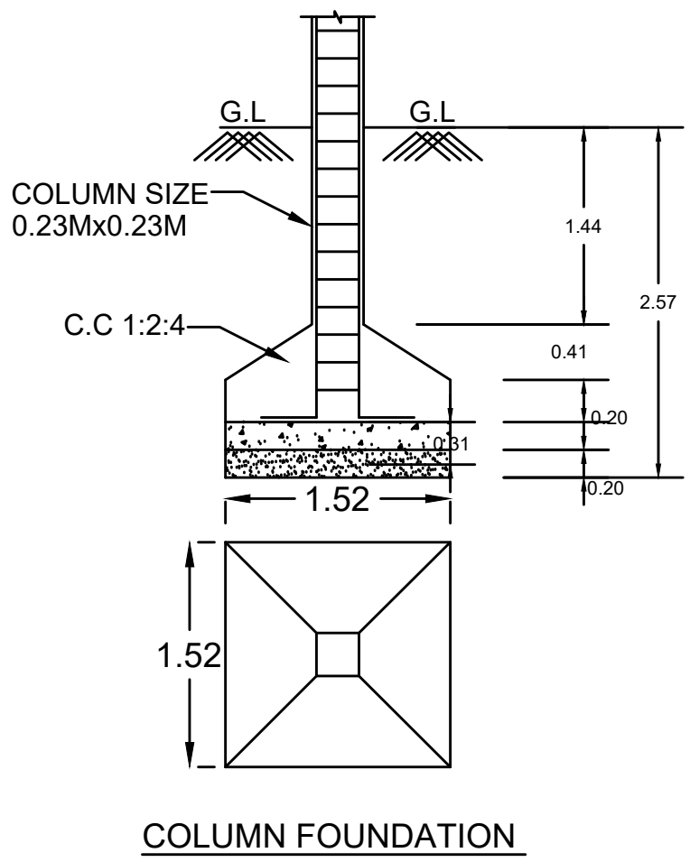
COLUMN FOUNDATION
