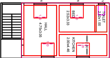
PROPOSED FIRST FLOOR PLAN
