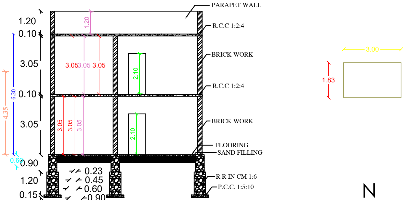
SECTION AB
