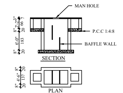
SEPTIC-TANK DETAIL
