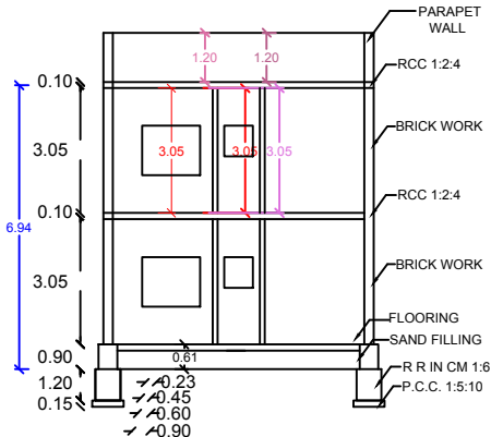
SECTION AB
