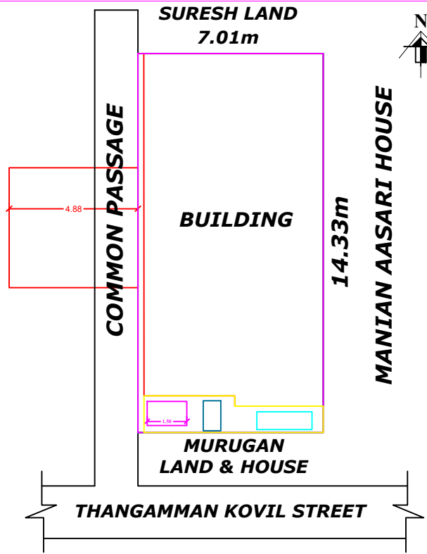
SITE PLAN
