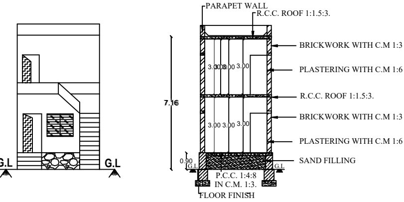
ELEVATION SECTION ON 'AA'
