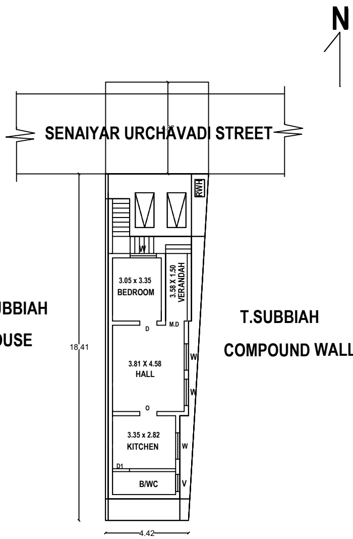
ADHILAKSHMI & SUBBIAH COMMON WALL SITE PLAN SCALE 1:100
