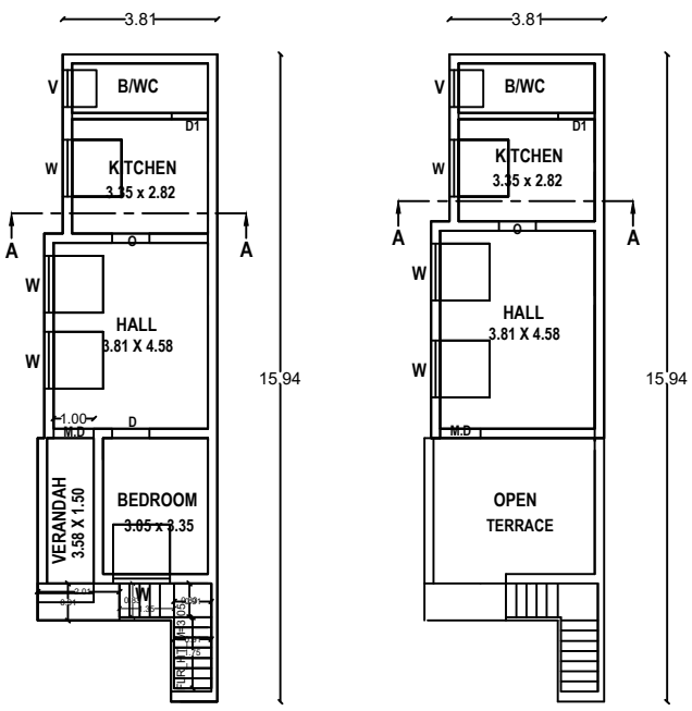
PLAN - GROUND FLOOR PLAN - FIRST FLOOR
