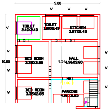
GF PLAN
