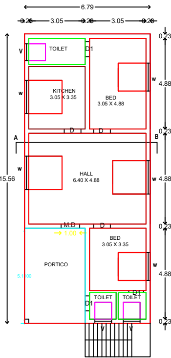
G.FLOOR PLAN
