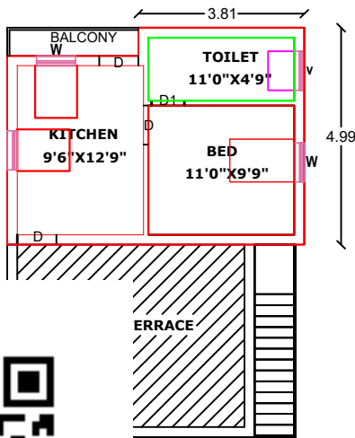
LOOR PLAN
