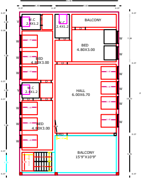
FIRST FLOOR RESIDENTIAL PLAN
