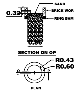
RAIN WATER PIT
