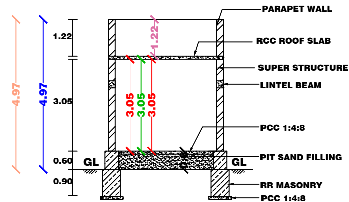
SECTION ON AB VELKUMAR SITE 17'0"
