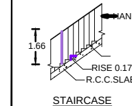
STAIRCASE
