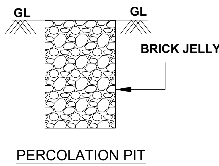
PERCOLATION PIT
