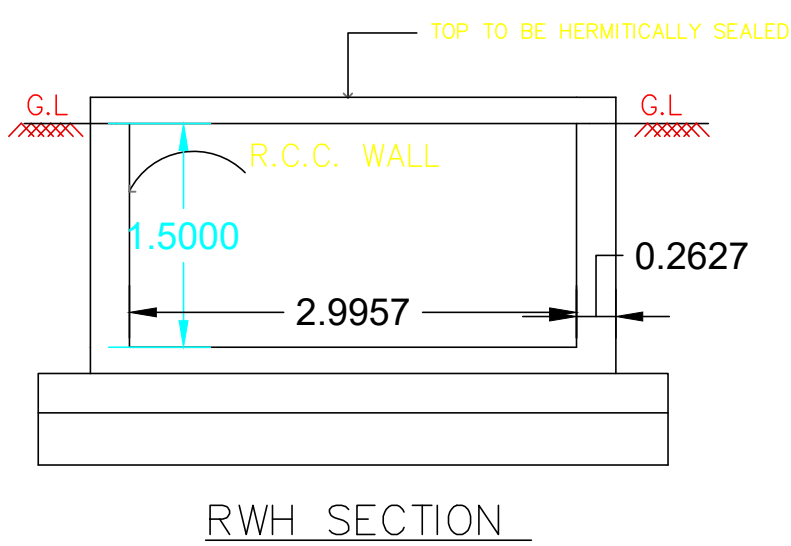
RWH SECTION
