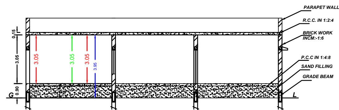
SECTION "AB"
