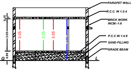
SECTION "AB"
