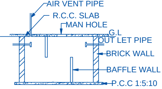
SECTION ON SEP.TANK
