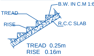
STAIR DETAILS
