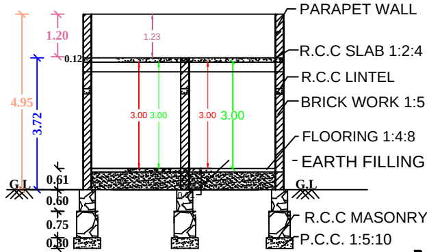
"SECTION "AB"
