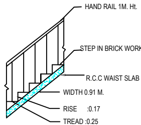
STAIR DETAIL
