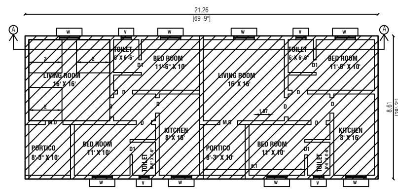
EX.GROUND FLOOR PLAN
