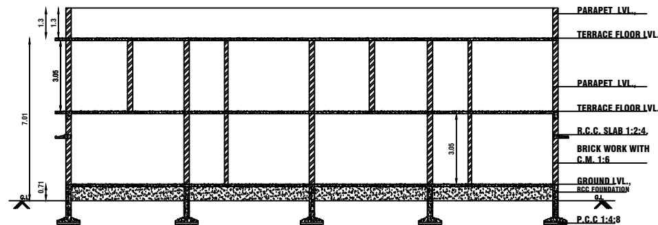
SECTION ON A-A & A'-A'
