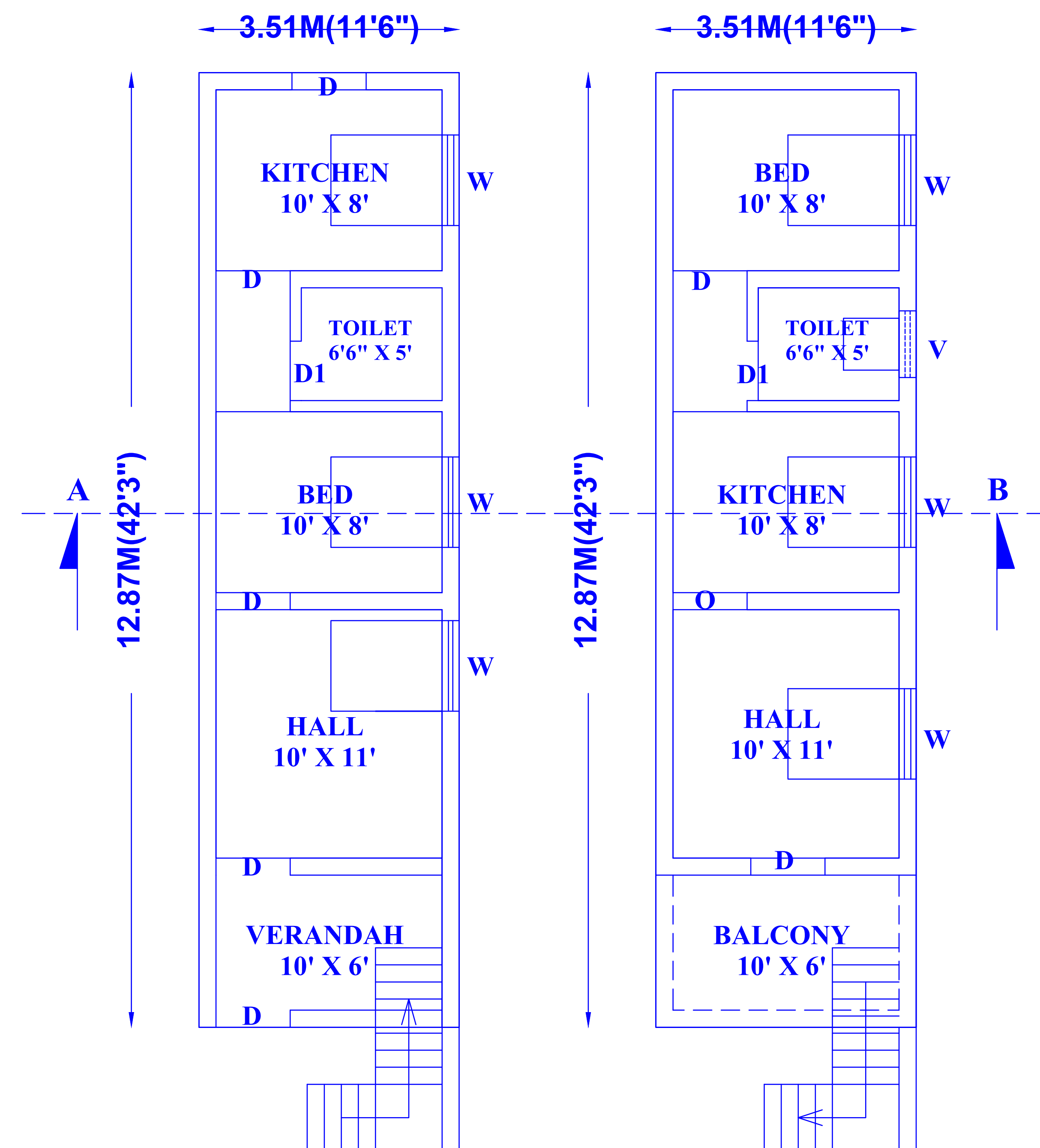
EX."GF"PLAN
