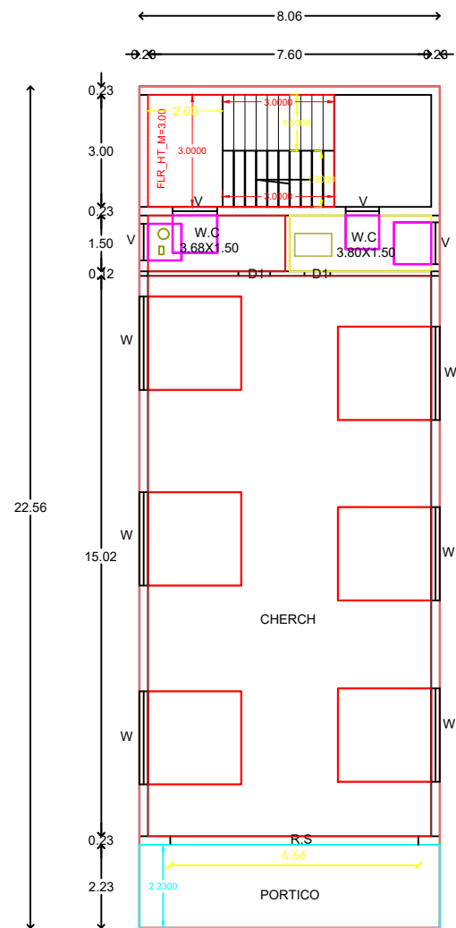
G.FLOOR PLAN
