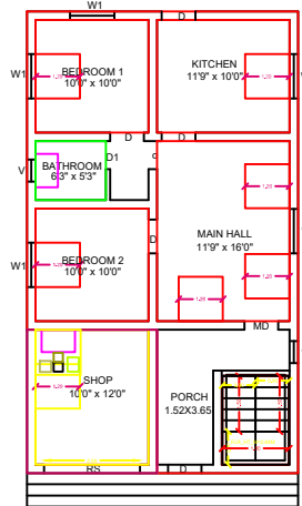
PLAN - GROUND FLOOR
