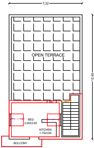
PLAN - FIRST FLOOR PROPOSED BUILDING
