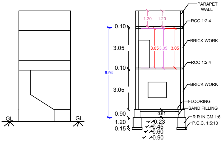
ELAVTION
