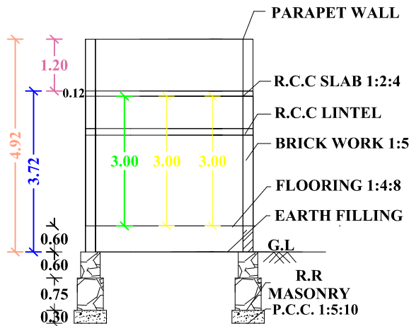
"SECTION "AB"
