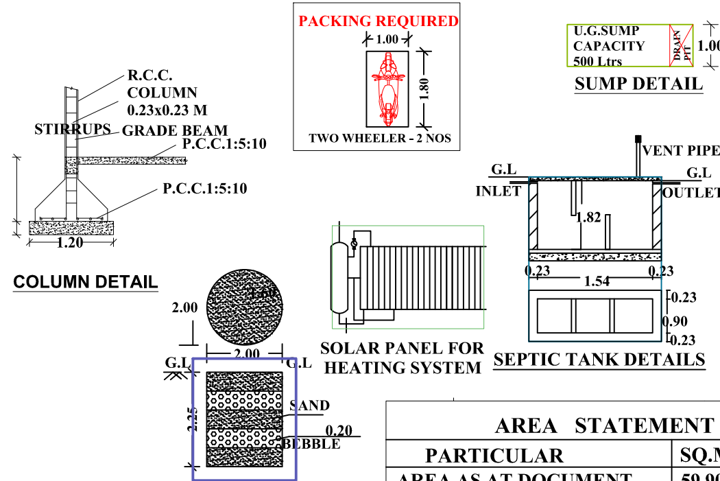
RAIN WATER HARVESTING
