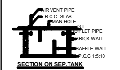
SECTION ON SEPTIC TANK
