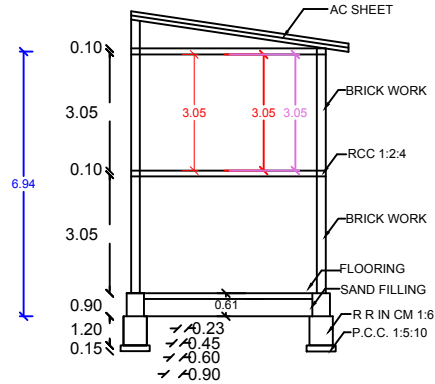
SECTION AB
