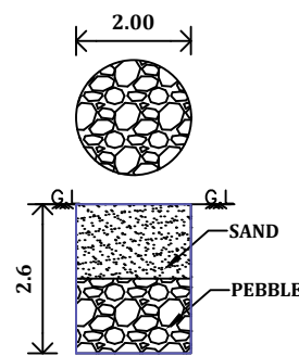
RAINWATER HARVESTING
