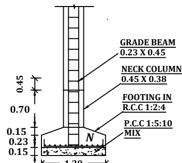
COLUMN DETAILS SCALE - 1:50
