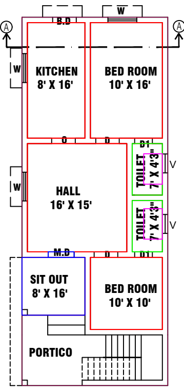
PLAN
