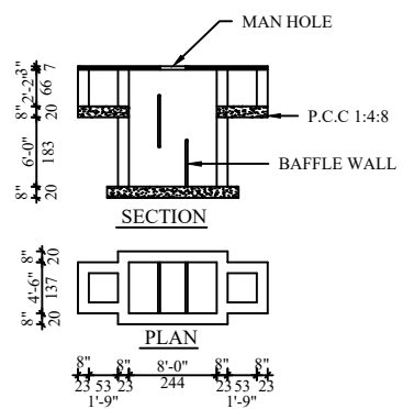
SEPTIC-TANK DETAIL
