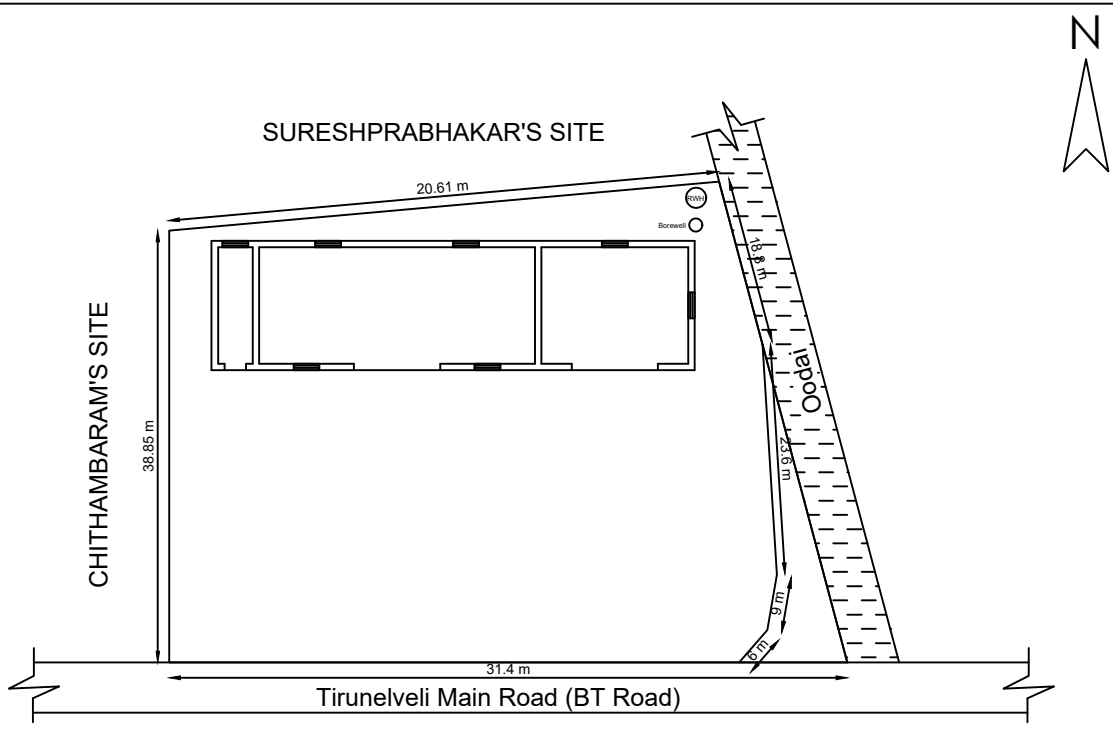
SITE PLAN
