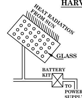
SOLAR SYSTEM
