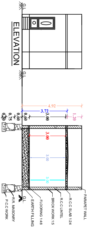
CROSS SECTION
