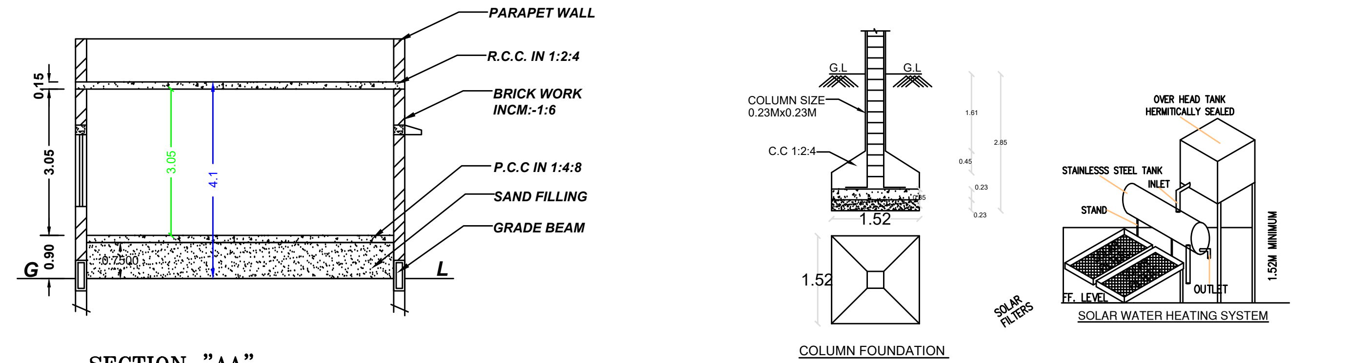
SECTION "AA"
