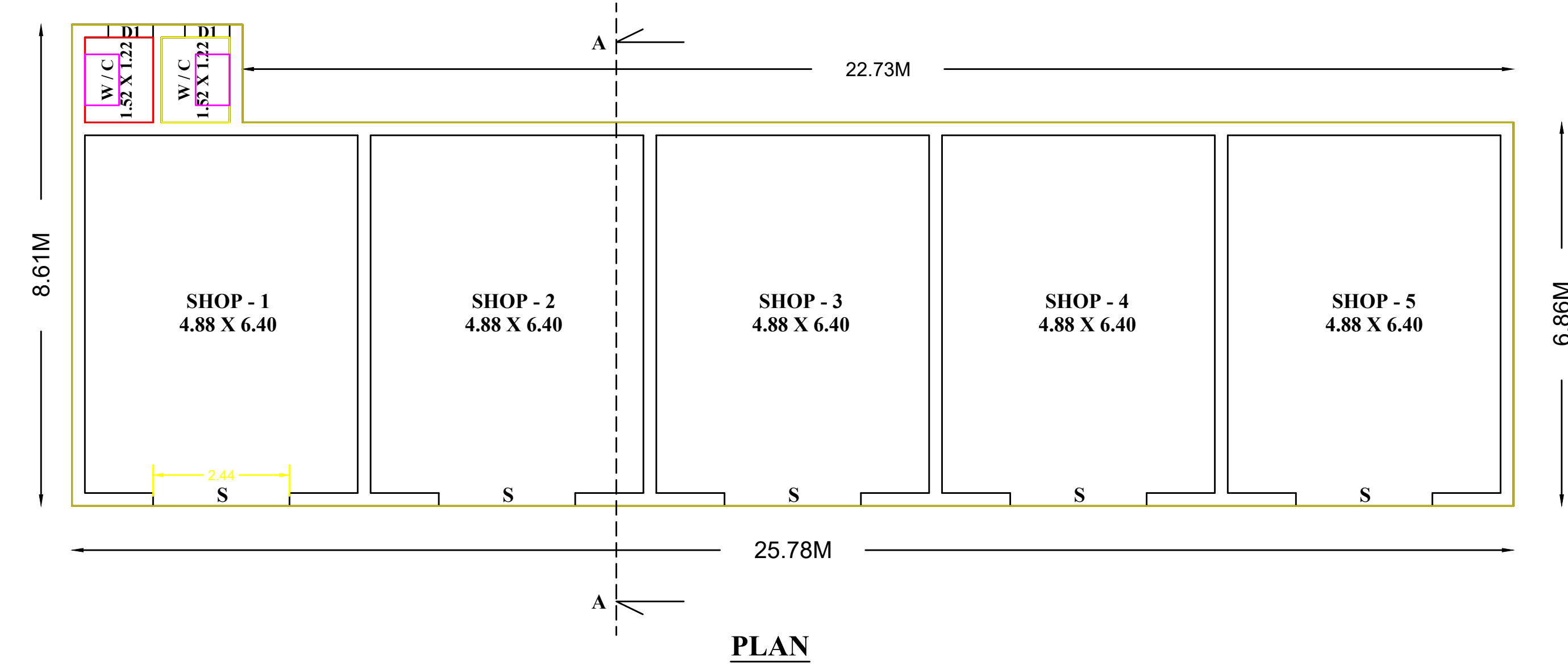
PLAN
