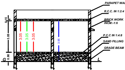
SECTION "AB"
