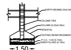
FOUNDATION DETAILS
