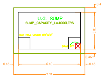
SUMP DETAIL SCALE 1"=4'0"
