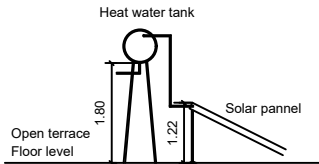
SIDE ELEVATION
