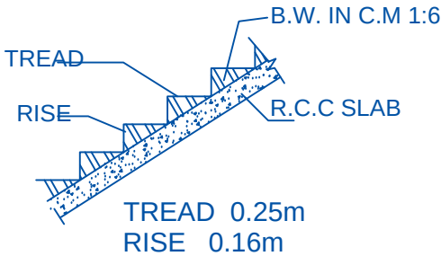
STAIR DETAILS
