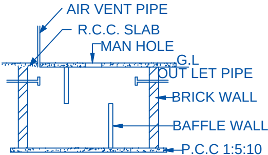
SECTION ON SEP.TANK
