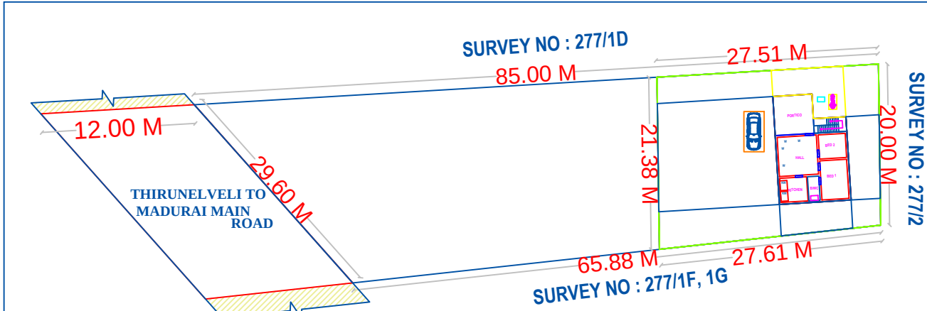
SITE PLAN SCALE:- 1:400
