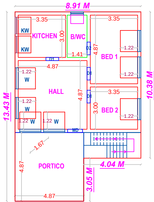
PLAN - GROUND FLOOR ( PROPOSED )
