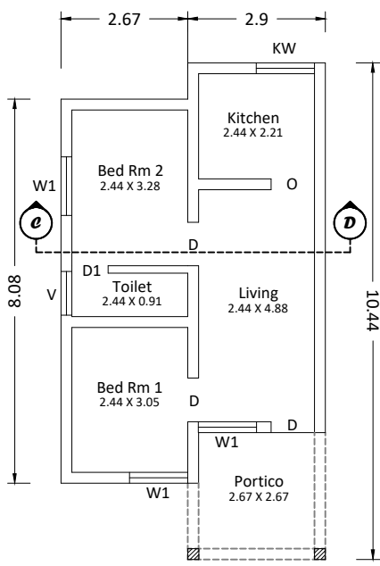
PLAN (HOUSE - 2)
