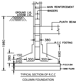
TYPICAL SECTION OF R.C.C. COLUMN FOUNDATION
