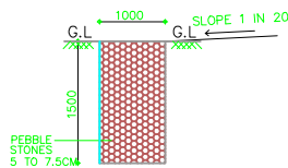
SECTION OF PEBBLE TRENCH
