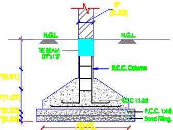
FOUNDATION DETAIL
