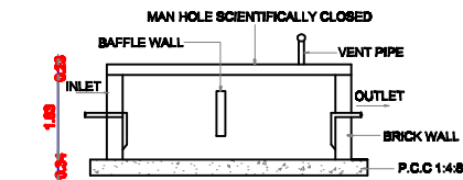
SECTION OF SEPTIC TANK
