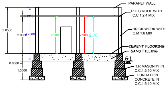
SECTION ON 'AB' SANKARALINGANADAR SITE 10.80 M
