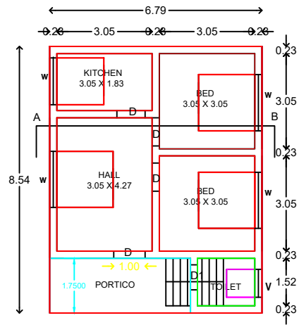
G.FLOOR PLAN
