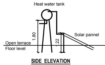
SIDE ELEVATION
