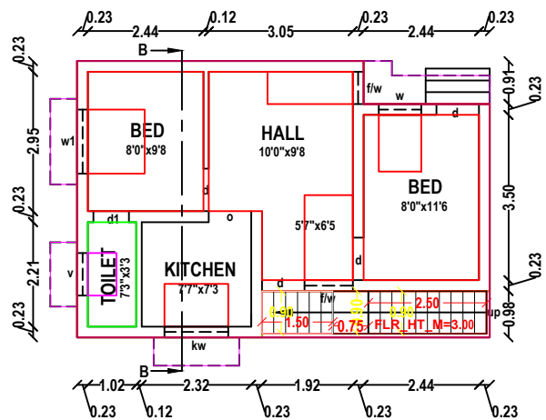
PLAN - GROUND FLOOR RESIDENCE
