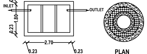
PLAN SEPTIC TANK DETAILS
