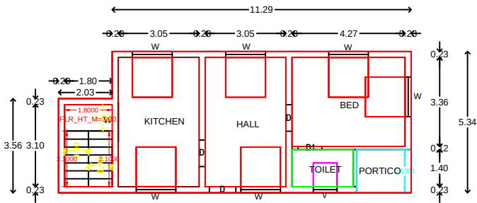
G.FLOOR PLAN
