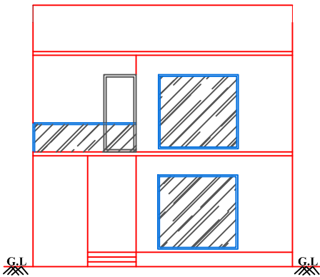
FRONT ELEVATION
