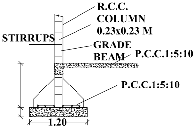
COLUMN DETAIL
