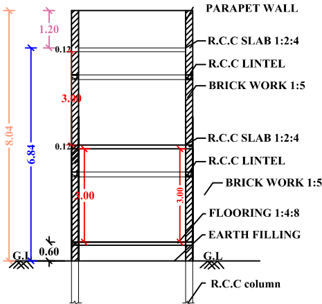
"SECTION "AB"
