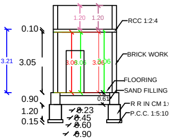
SECTION AB
