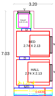
PLAN
