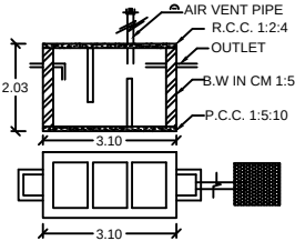
SEPTIC TANK AND TRENCH
