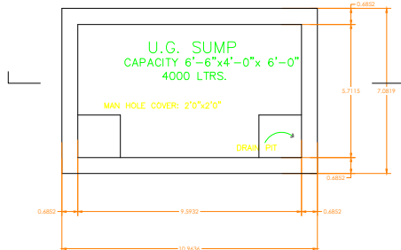
SUMP DETAIL SCALE 1"=4'-0"
