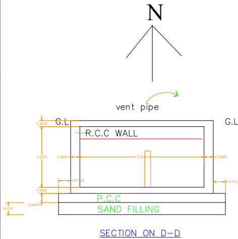
SECTION ON D-D
