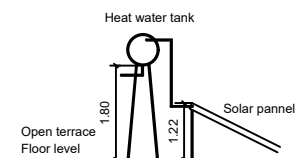
SIDE ELEVATION
