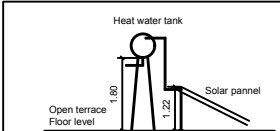
SIDE ELEVATION
