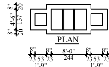
SEPTIC-TANK DETAIL
